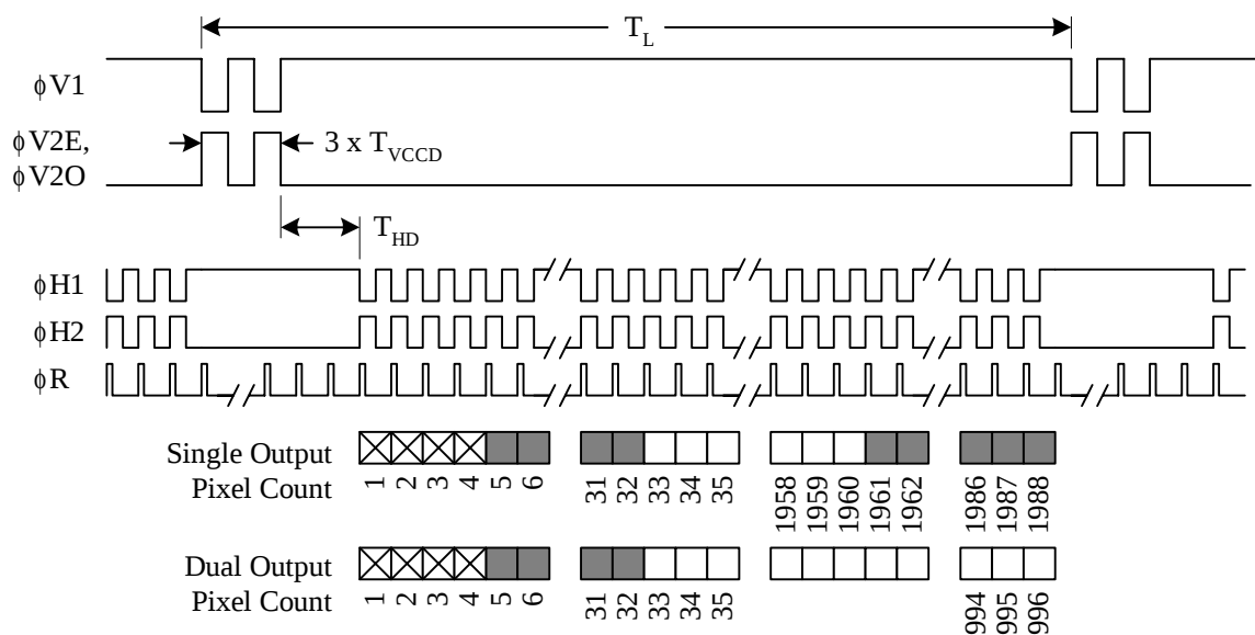
Figure 8 - Line Timing
