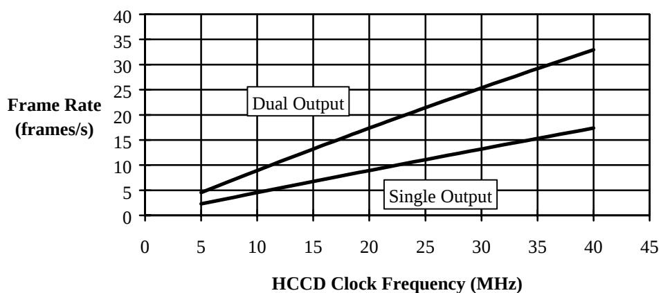
Figure 10 - Progressive Frame Rate vs. HCCD Clock Frequency
