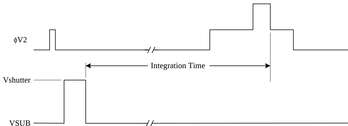
Figure 9 - Electronic Shutter Timing Diagram
