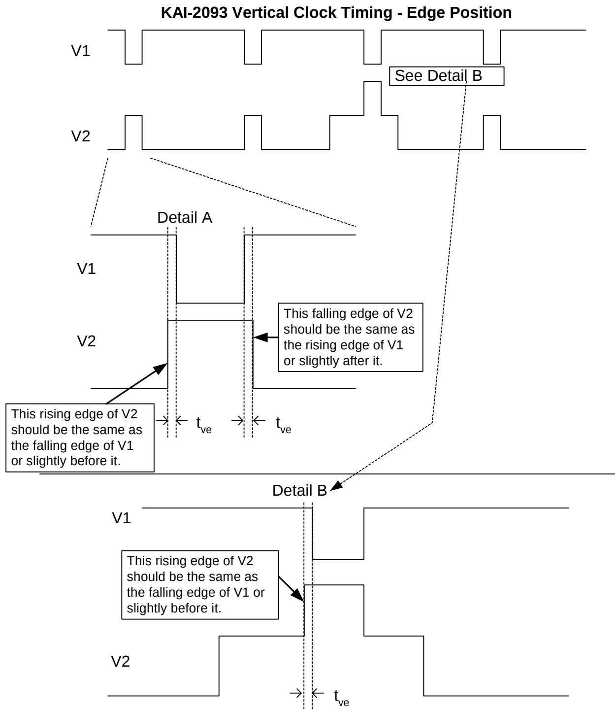
Figure 5 - Ideal Vertical Clock Edge Position
