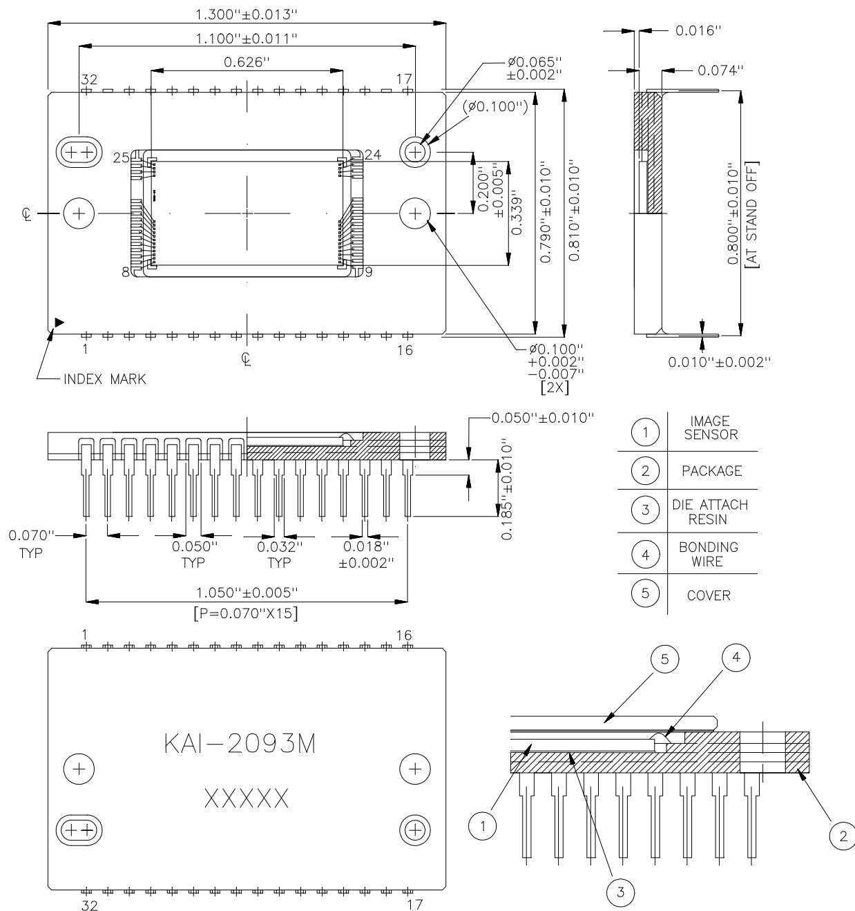
Figure 2 - Package Drawing
